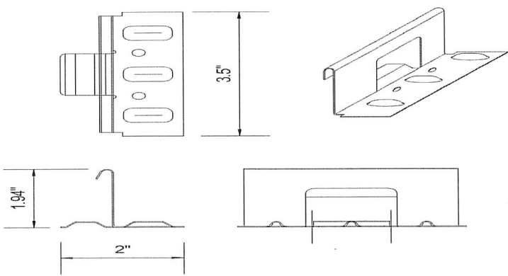
18 GA Galvanized Clip
